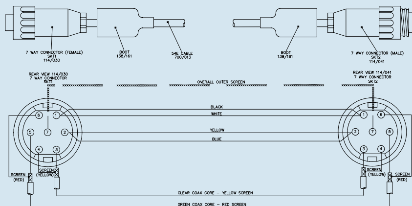
Cable Assembly 138/332
