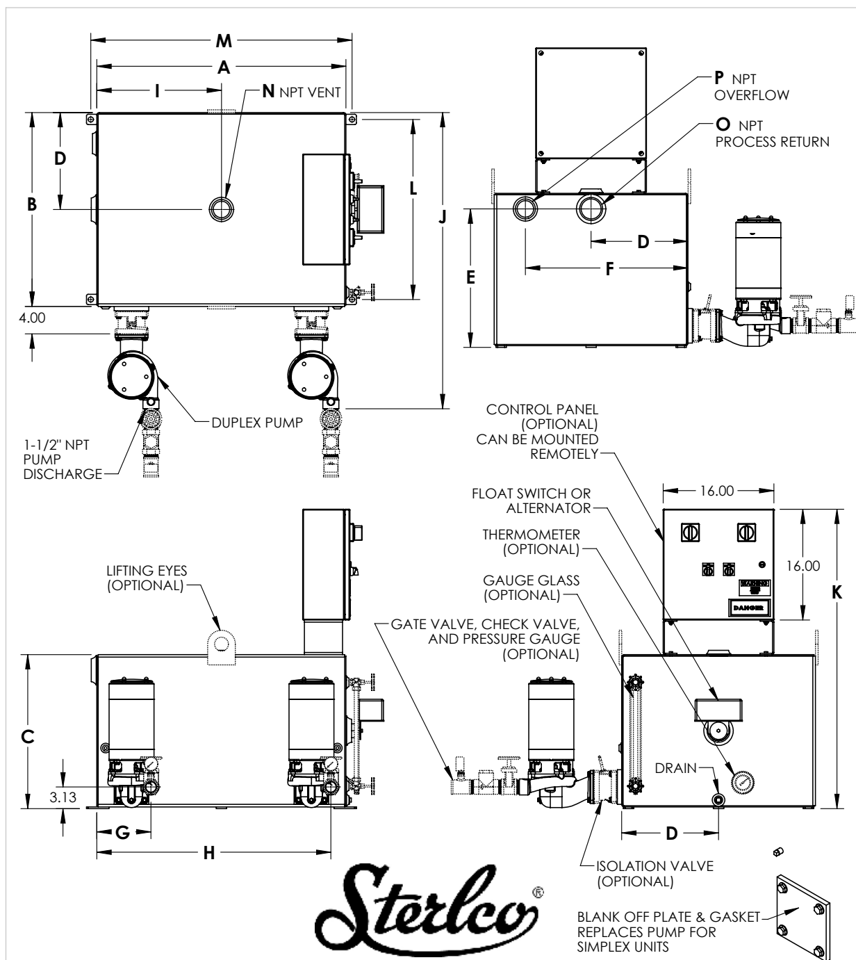
4800 "K" SERIES CONDENSATE UNIT RECEIVER MATERIAL: STAINLESS STEEL
