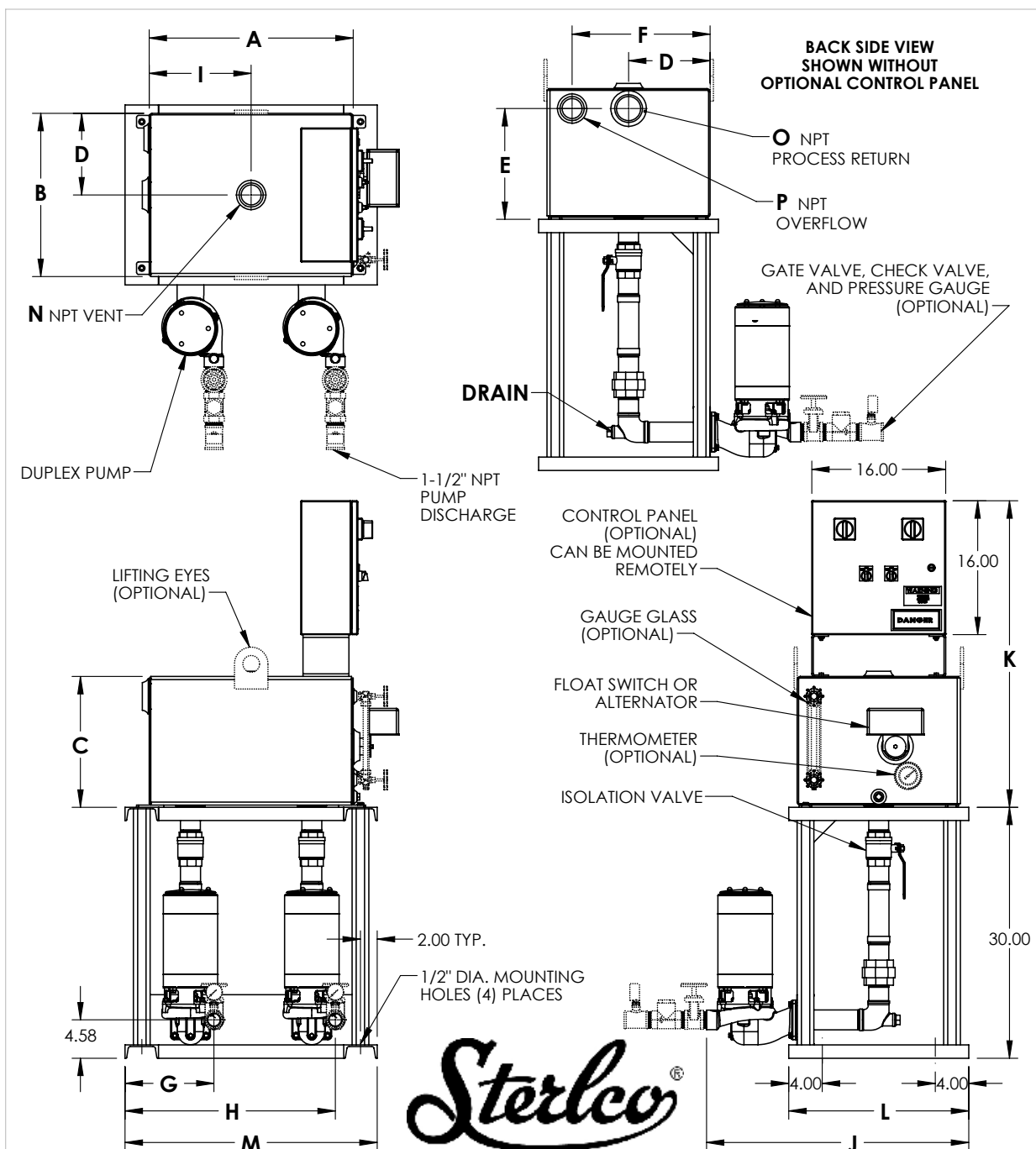
4800 "K" SERIES ELEVATED CONDENSATE UNIT RECEIVER MATERIAL: STAINLESS STEEL
